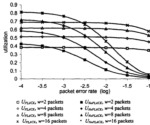
Fig. 6. Utilization versus packet error rate for various window sizes, l=16 Kbits, C_p=2.8 msec, T_i=5 sec, C=4 Mbit/s.
