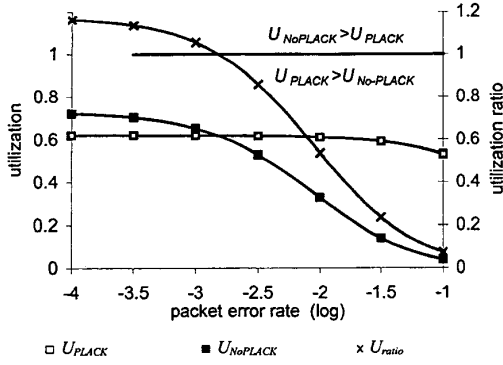
Fig. 3. Utilization and utilization ratio versus packet error rate, w=8 packets, l=16 Kbits, C_p=2.8 msec, T_l=5 sec, C=4 Mbit/s.
