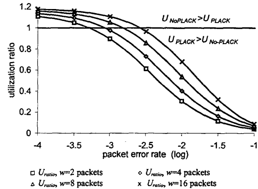
Fig. 7. Utilization ratio versus packet error rate for various window sizes, l=16 Kbits, C_p=2.8 msec, T_i=5 sec, C=4 Mbit/s.
