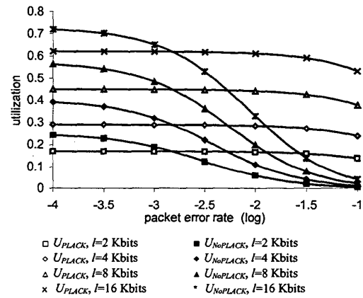
Fig. 8. Utilization versus packet error rate for various packet sizes, w=8 packets, C_p=2.8 msec, T_i=5 sec, C=4 Mbit/s.
