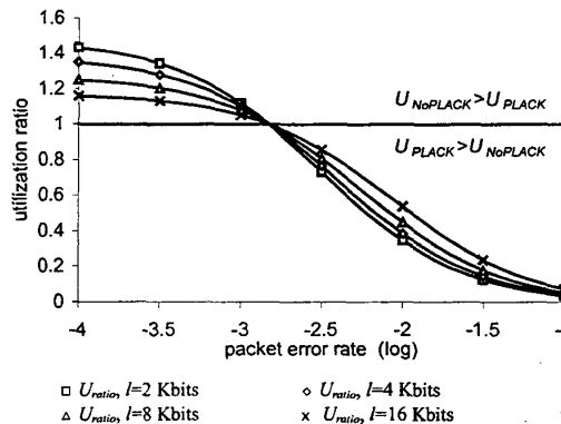
Fig. 9. Utilization ratio versus packet error rate for various packet sizes, w=8 packets, C_p=2.8 msec, T_f=5 sec, C=4 Mbit/s.
