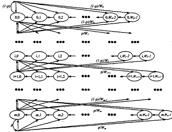
Fig. 2. Markov Chain model for backoff CW
