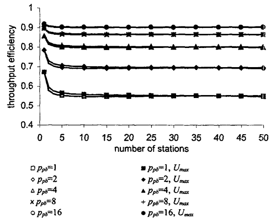
Fig. 7. Throughput efficiency versus n , l=16 Kbits, W=1 , m=20 , C=4 Mbit/s
