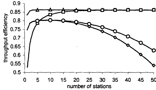
Fig. 3. Throughput efficiency: analysis versus simulation, l=16 Kbits, C=4 Mbit/s
