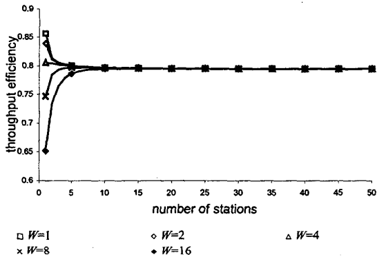
Fig. 6. Throughput efficiency versus n , m=62 , l=16 Kbits, p_{pb}=4 , C=4 Mbit/s.
