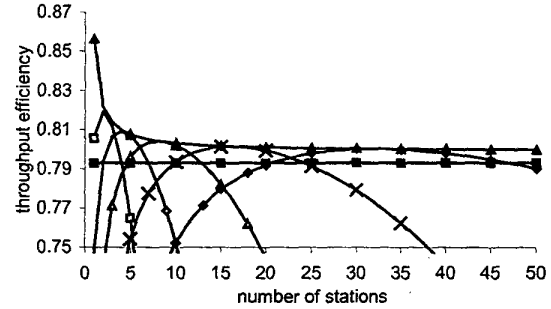
Fig. 4. Throughput efficiency versus n for fixed CW size, l=16 Kbits, p_{pb}=4 , C=4 Mbit/s.
