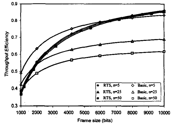
Fig. 5 Throughput versus frame size for C=1 Mbps
