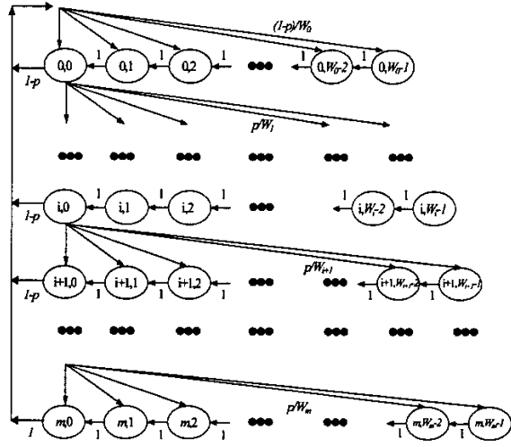
Fig. 4 Markov chain model
