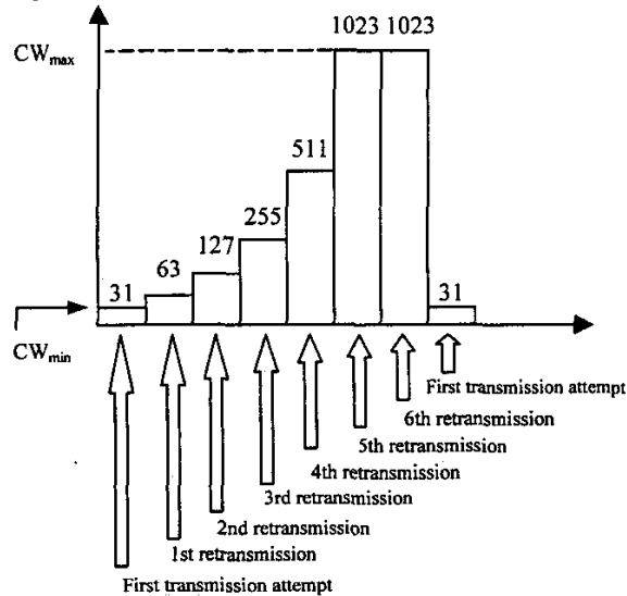
Fig. 3 The exponential increase of CW
