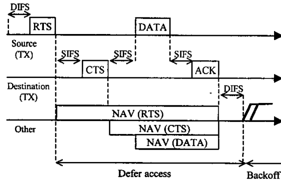
Fig. 2 RTS/CTS mechanism
