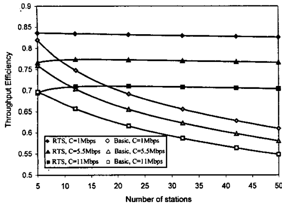
Fig. 6 Throughput versus number of stations
