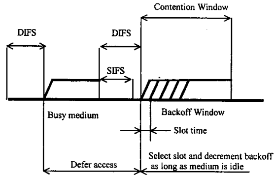
Fig. 1 Basic Access mechanism
